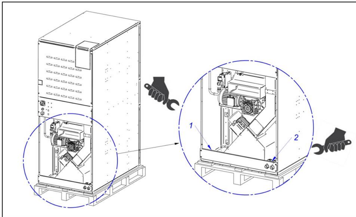
- LOCATION OF BOLTS 1 AND 2 - UNSCREW USING A FLAT NO 13 SPANNER
